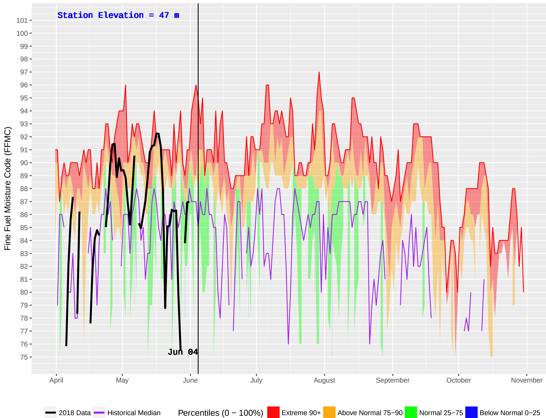
HAGENSBORG 2 (904) : Historical (2005–2016) and Current (2018) Noon Fine Fuel Moisture Code (FFMC)
