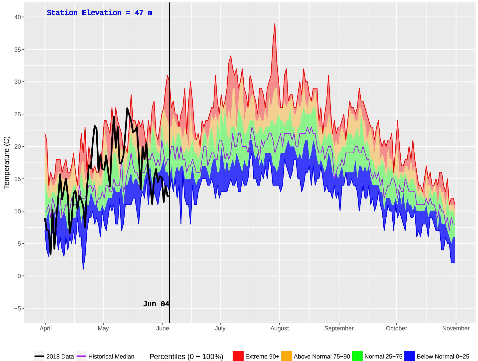
HAGENSBORG 2 (904) : Historical (2005–2016) and Current (2018) Noon Temperature
