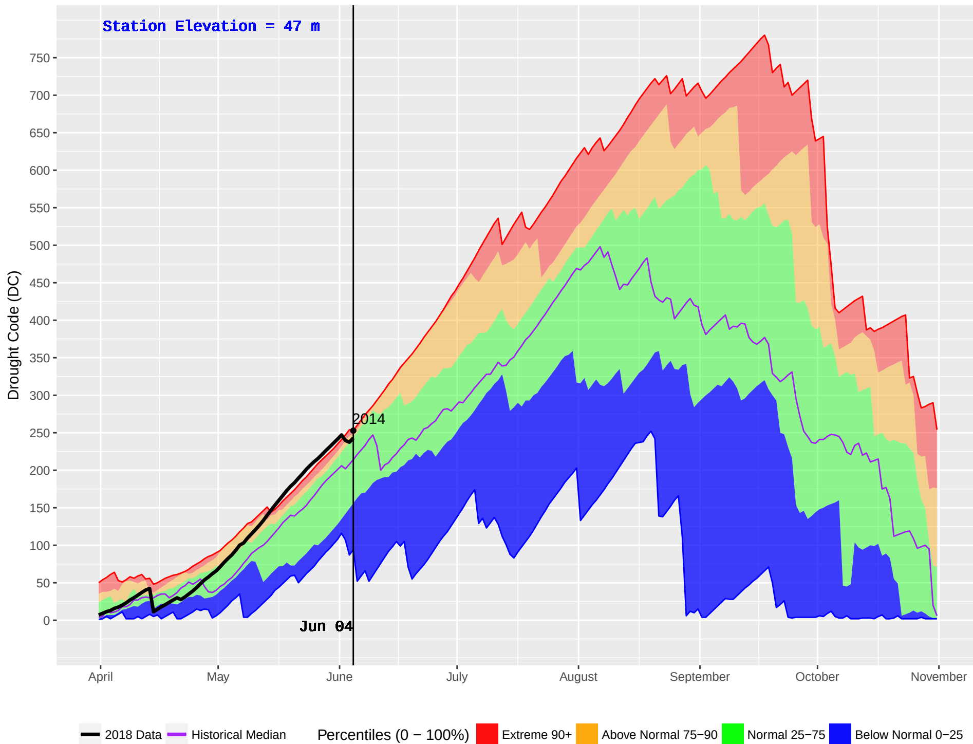
HAGENSBORG 2 (904) : Historical (2005–2016) and Current (2018) Noon Drought Code (DC)
