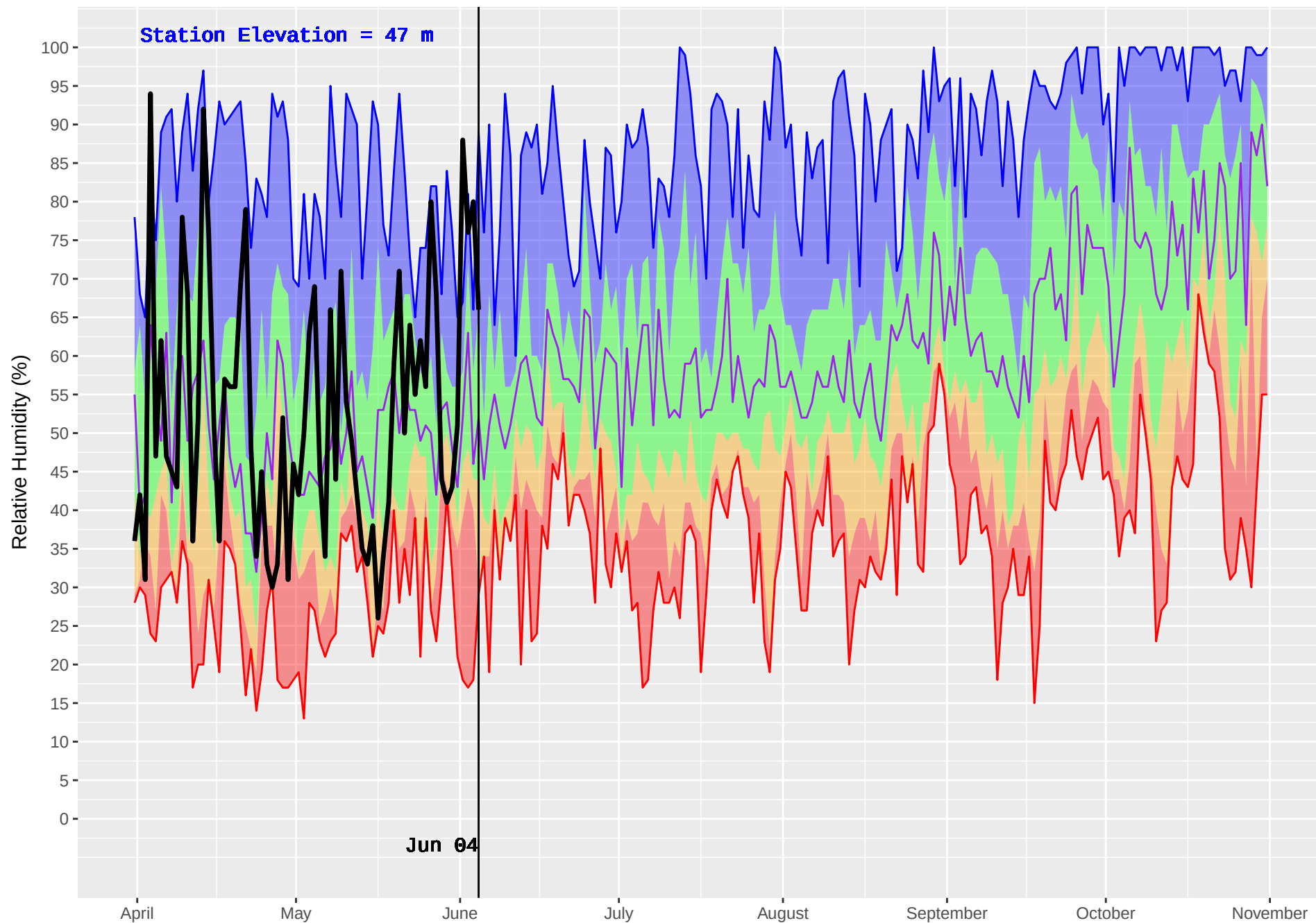
HAGENSBORG 2 (904) : Historical (2005–2016) and Current (2018) Noon Relative Humidity
