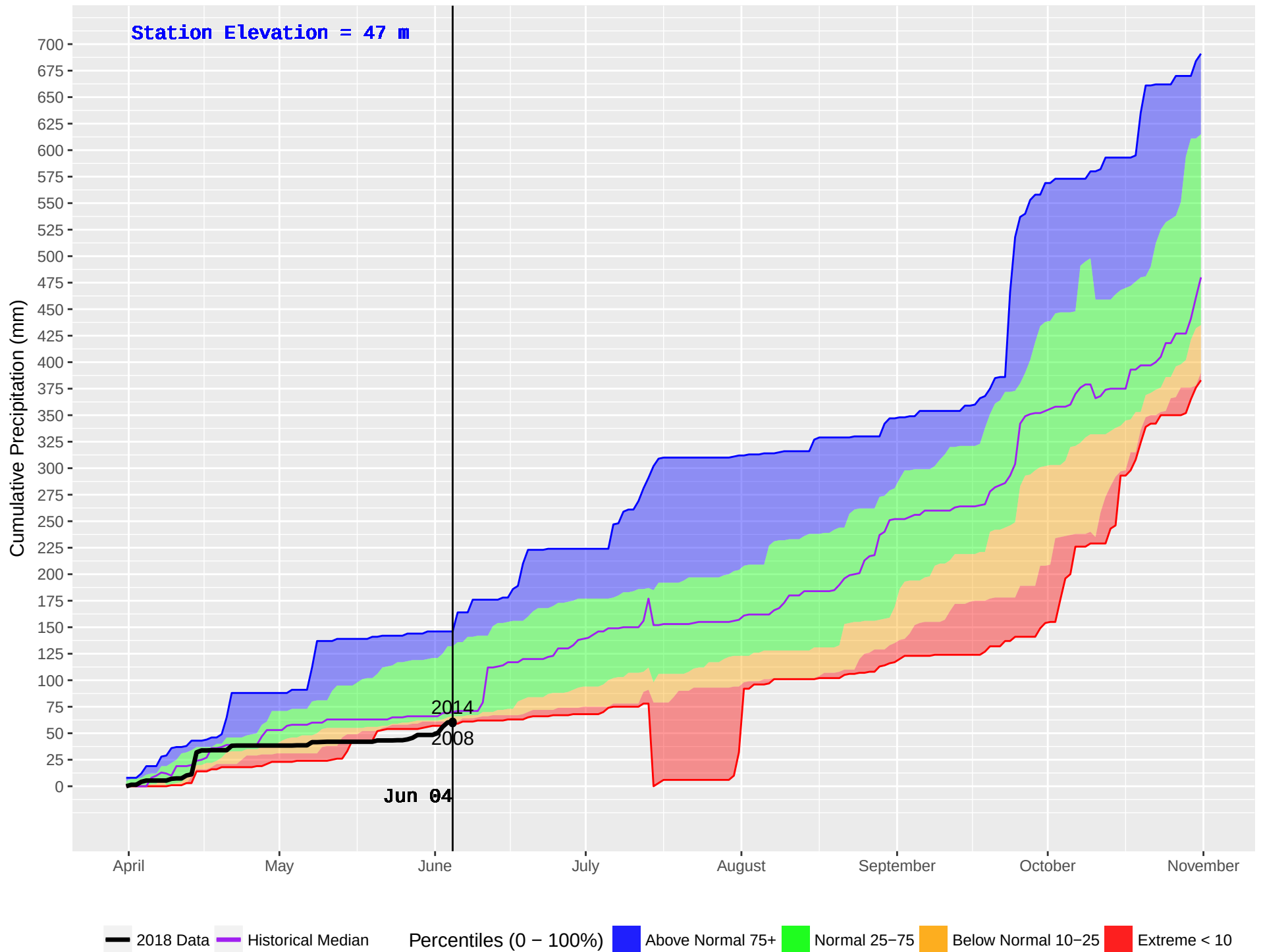
HAGENSBORG 2 (904) : Historical (2005–2016) and Current (2018) Noon Cumulative Precipitation
