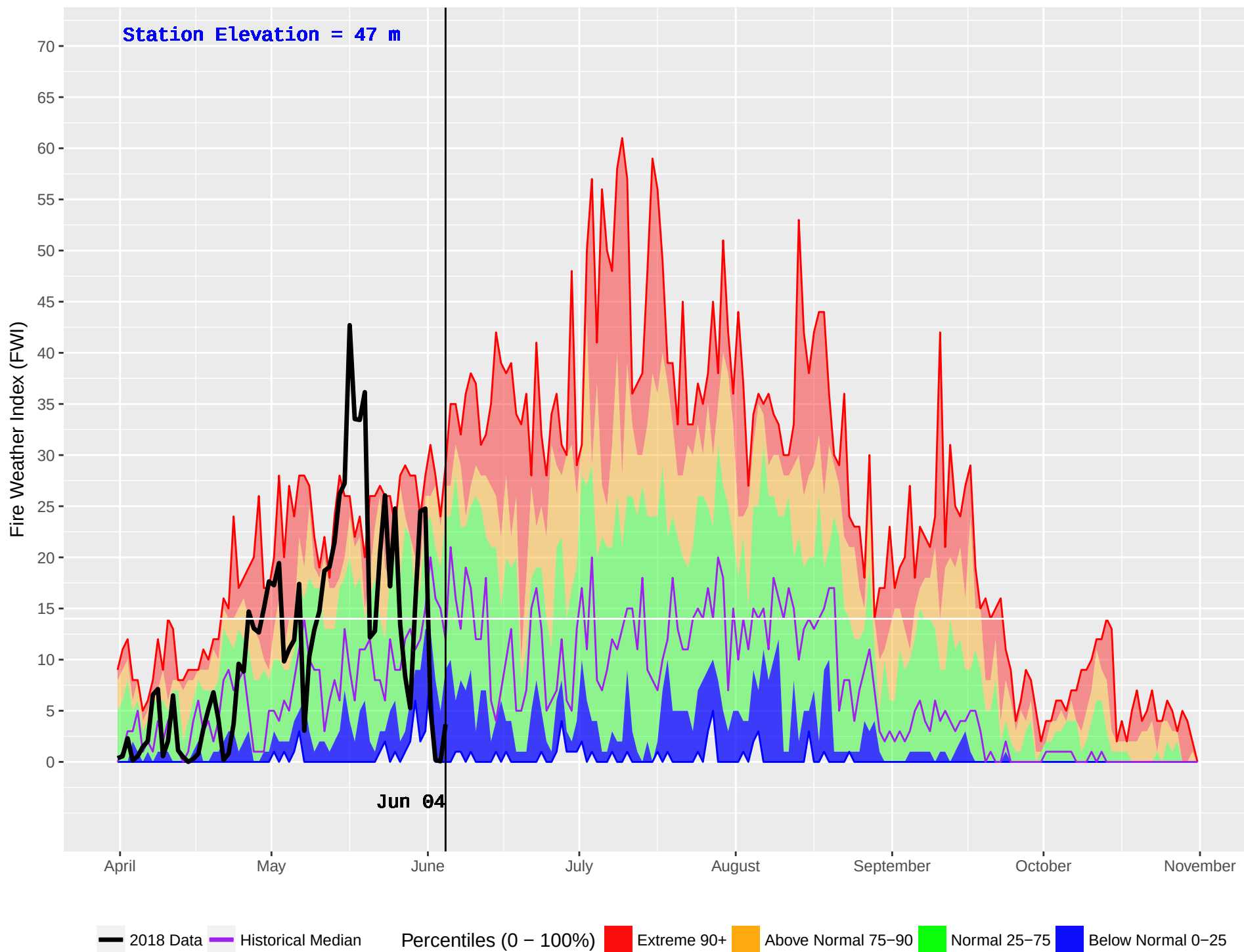
HAGENSBORG 2 (904) : Historical (2005–2016) and Current (2018) Noon Fire Weather Index (FWI)
