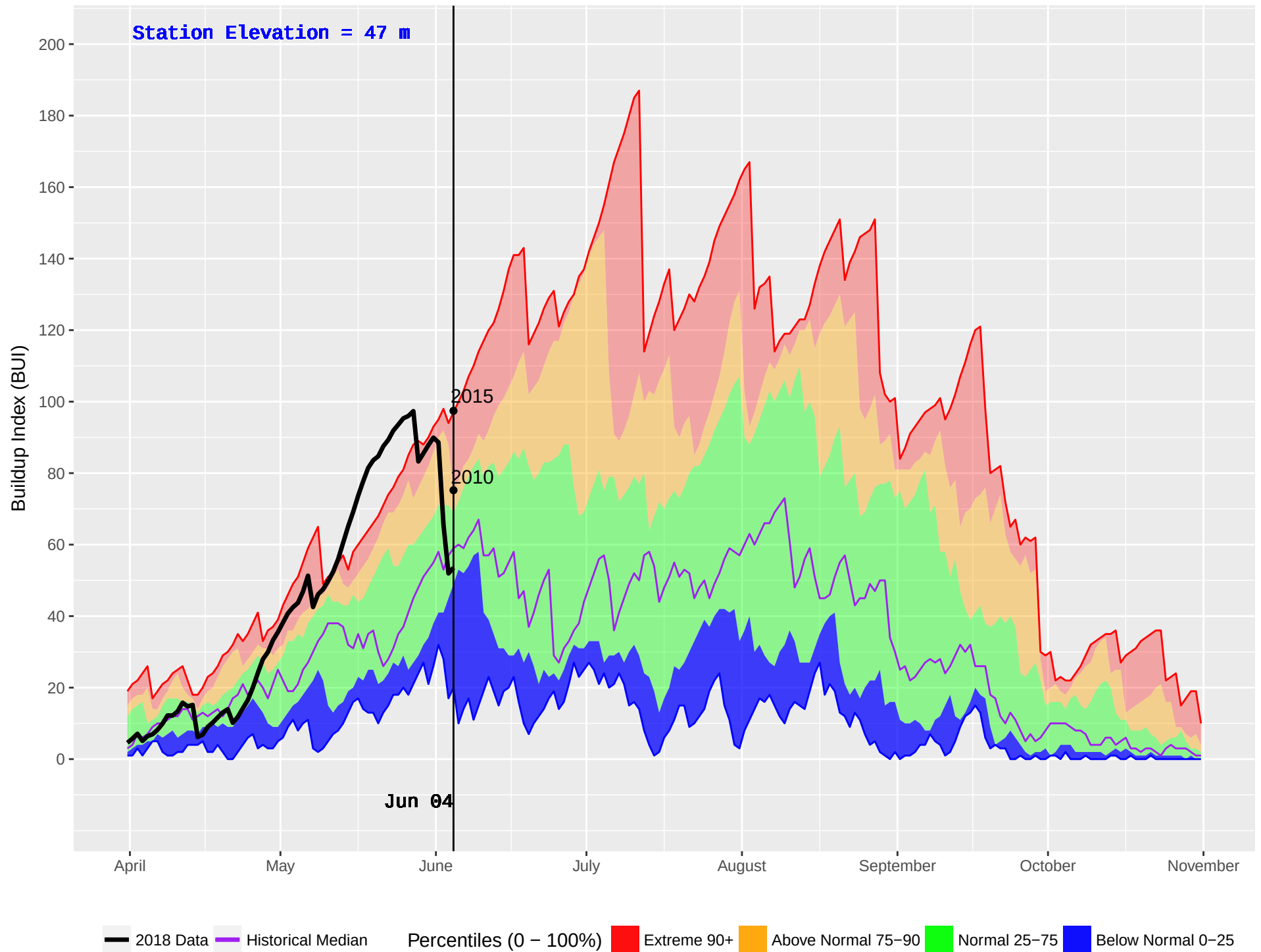
HAGENSBORG 2 (904) : Historical (2005–2016) and Current (2018) Noon Buildup Index (BUI)
